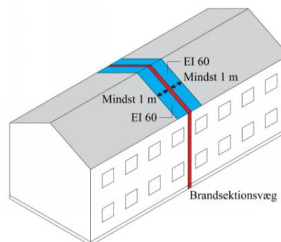
Figur 5 – Illustration af brandkamserstating (Figur 4.14 i BR18, Kapitel 5)
